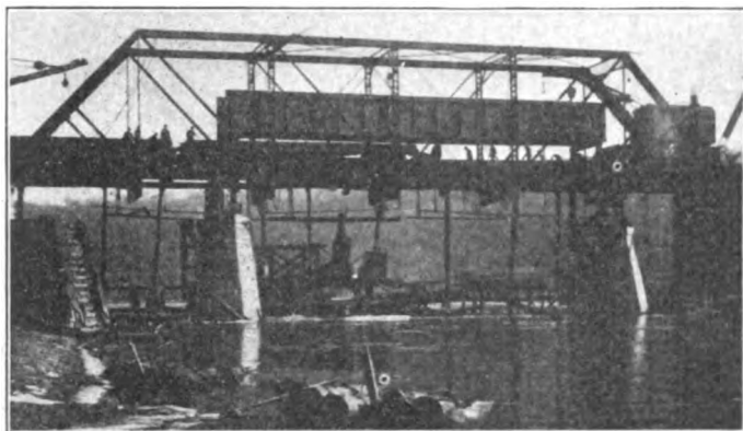
Erecting One of the 80-ft. Girder Spans
