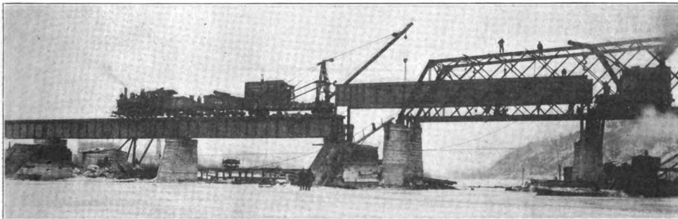
Girders of 100-ft. Span Resting on Temporary Bents While Intermediate Pier Is Being Cut Down
