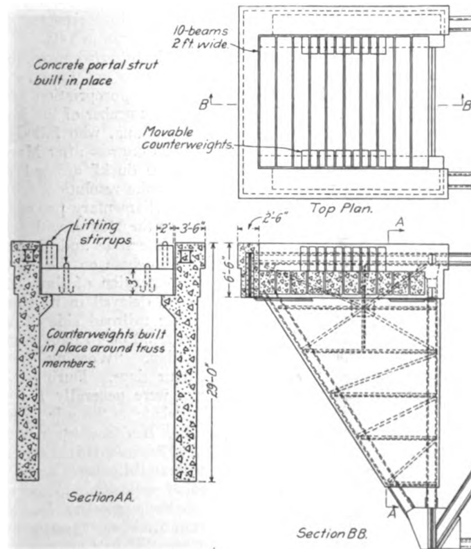
Details of the Reinforced Concrete Counterweight
